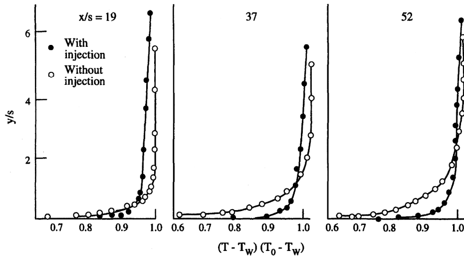
Fig. 11. Temperature profiles behind the recirculation zone.
