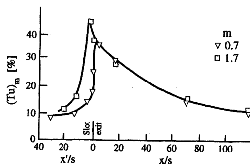
Fig. 7. Change of the maximum turbulence degree along the channel wall.
