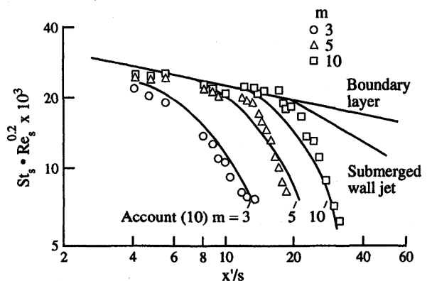
Fig. 12. Heat transfer of a counter-current wall jet on the basic part of its development.
