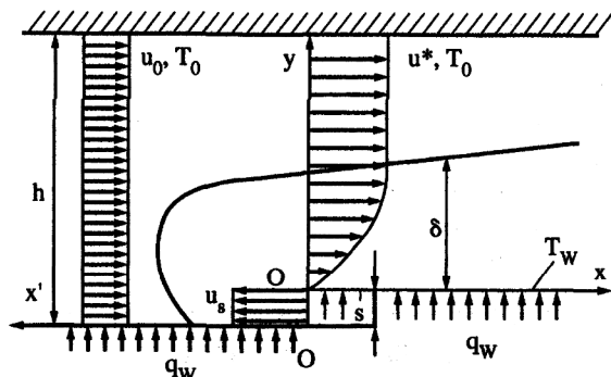
Fig. 1. Scheme of a counter-current wall jet flow.
