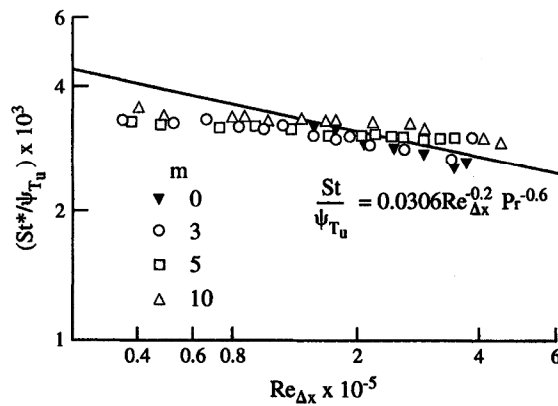
Fig. 13. Generalization of experimental data on heat transfer behind the recirculation zone.
