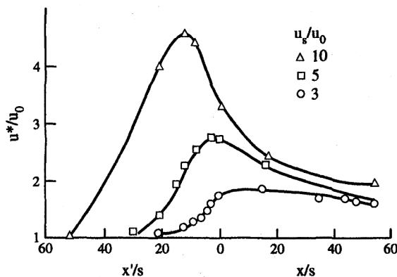
Fig. 6. Velocity increase in the flow core.
