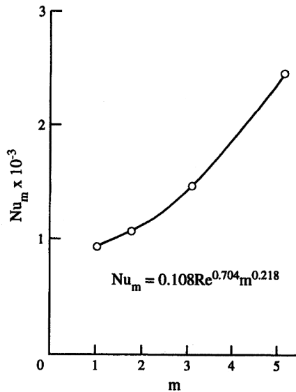
Fig. 10. Influence of the injection intensity on Nu_m behind the place of a counter and normal injection.
