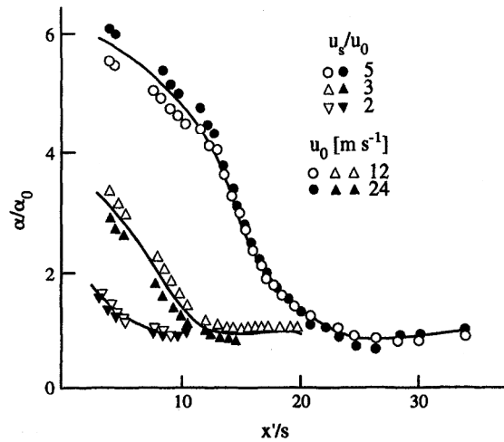
Fig. 8. Distribution of relative heat transfer coefficients in the area of a counter-current wall jet propagation.
